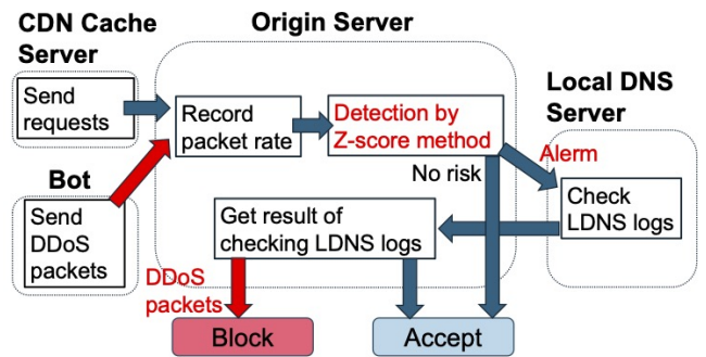
図 2 Flow of proposed method checking log of LDNS servers
