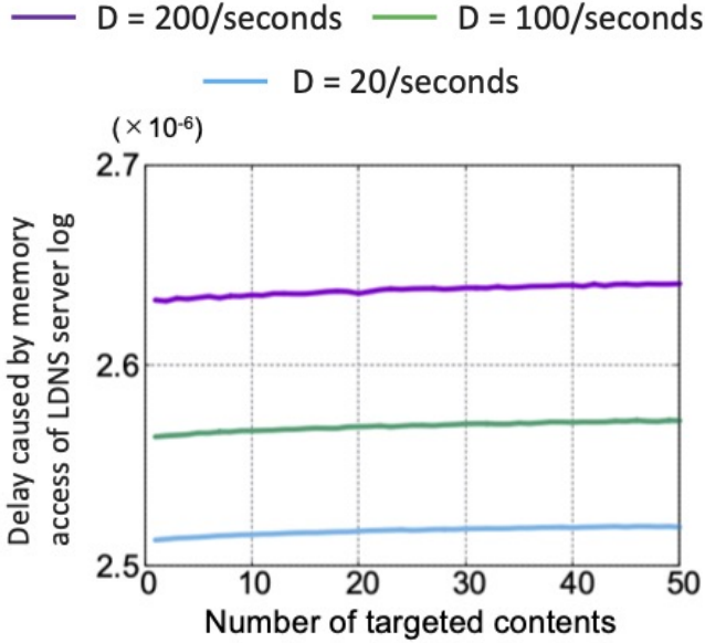
図 4 Delay caused by memory access of LDNS server log
