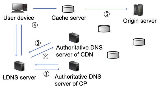
図 1 Name resolution procedure using DNS
