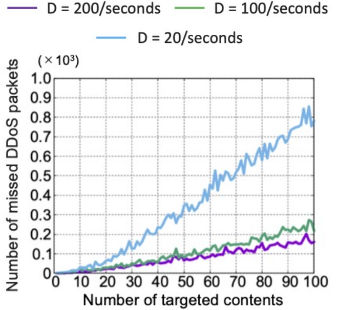
図 5 Number of undetected DDoS packets against number of targeted contents
