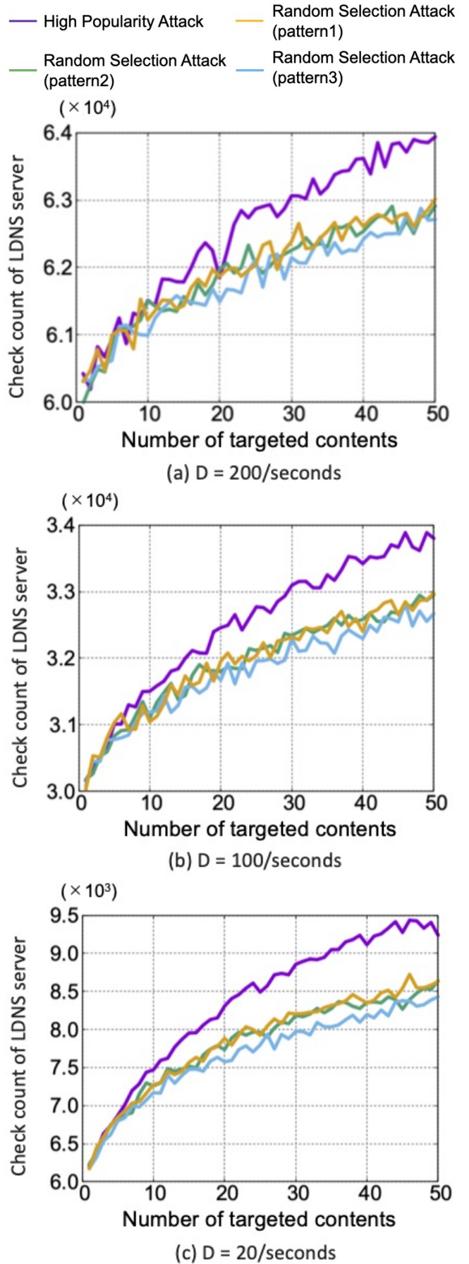
図 3 Total number of checks of LDNS server
