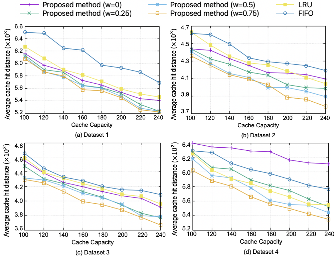
図 4.4: Average cache hit distance against cache capacity
