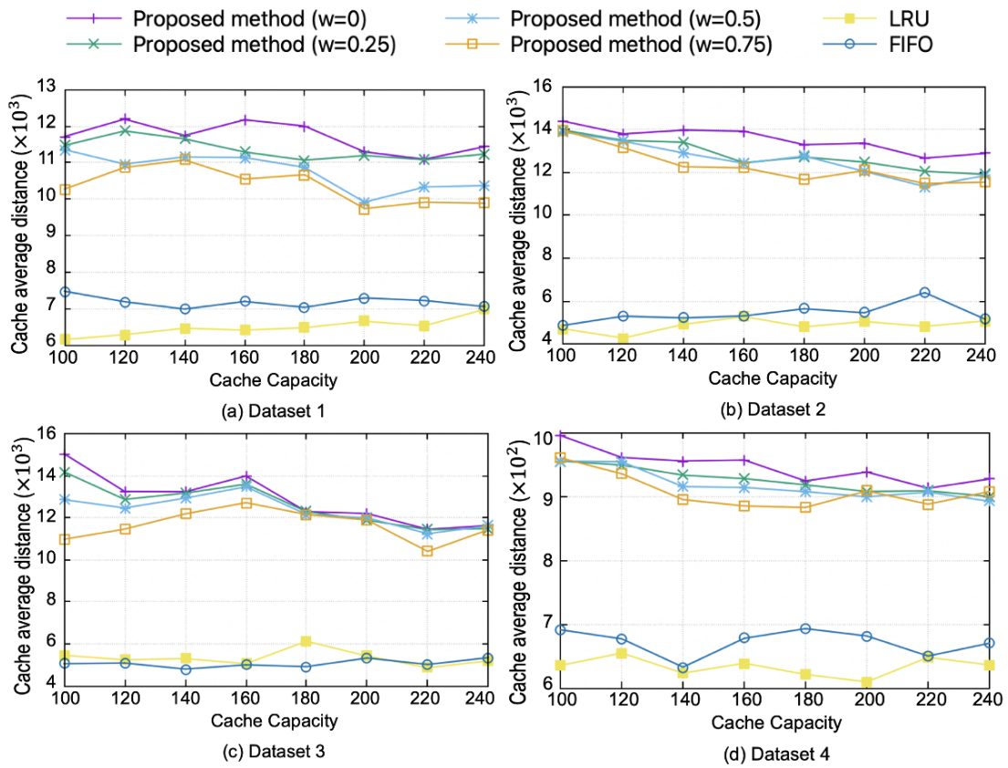
図 4.3: Cache average distance against cache capacity
