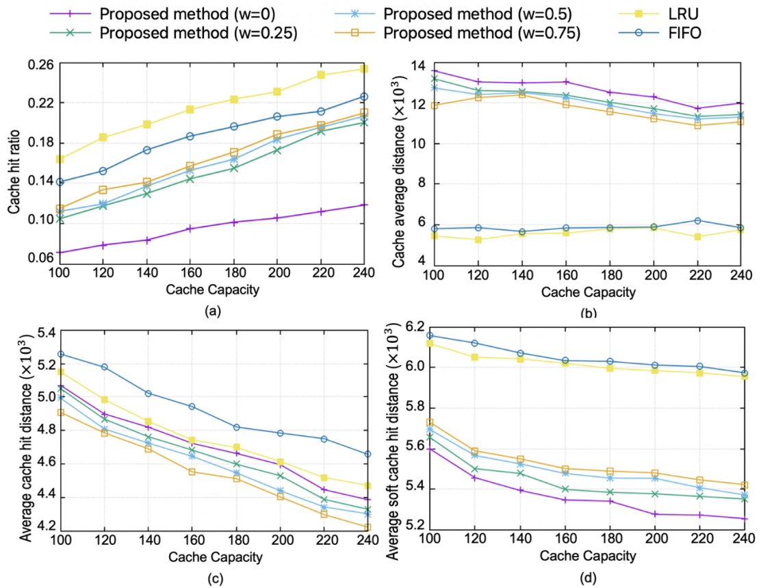
図 4.6: (a) Cache hit ratio, (b) cache average distance, (c) average cache hit distance, and (d) average soft cache hit distance, against cache capacity when mixing three datasets
