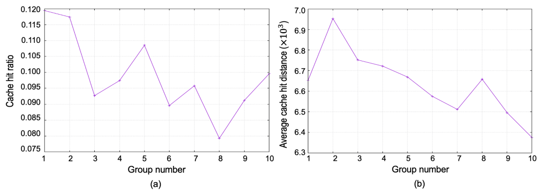
図 4.7: (a) Cache hit ratio and (b) average cache hit distance against cache group number
