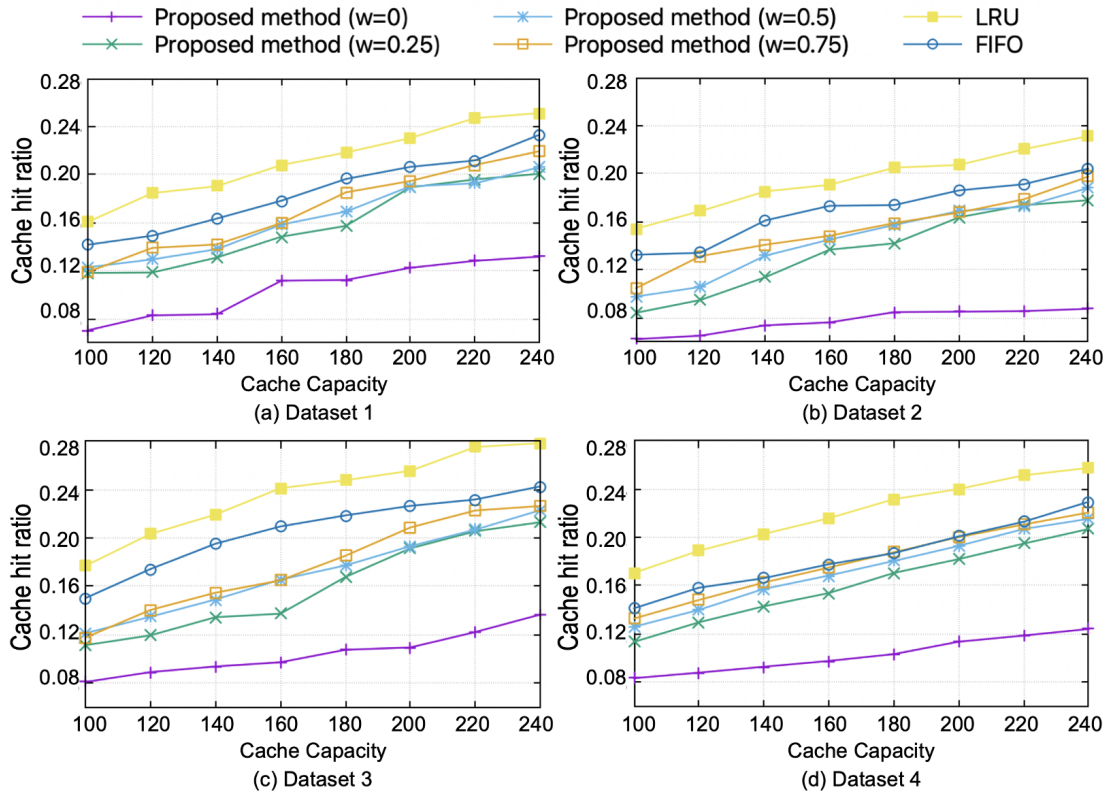
図 4.2: Cache hit ratio against cache capacity
