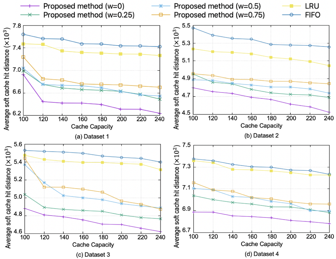
図 4.5: Average soft cache hit distance against cache capacity
