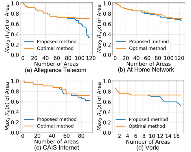
図 7 Max_2 R_n(x) of each area selected by each method in descending order when setting T = 0.7
