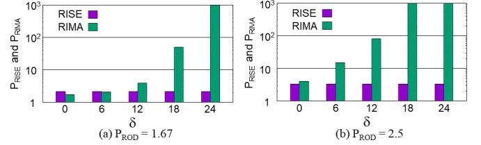
Fig. 5. Value of p satisfying F = F_{ROD} in RISE and RIMA
